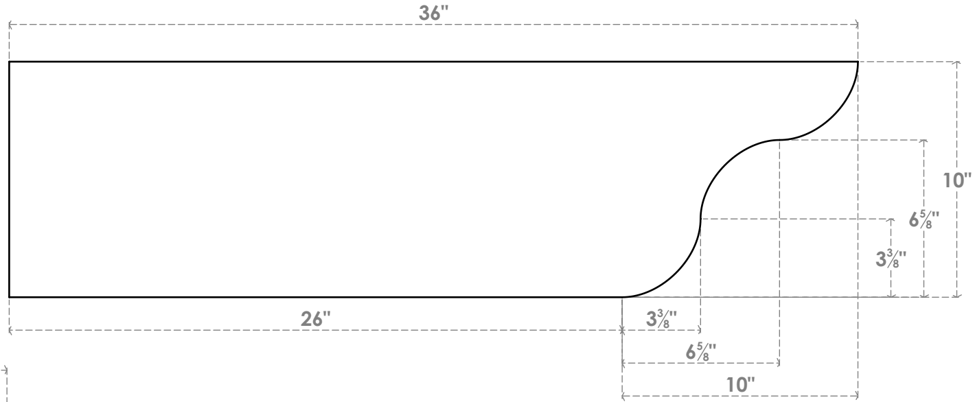
SIDE PROFILE
